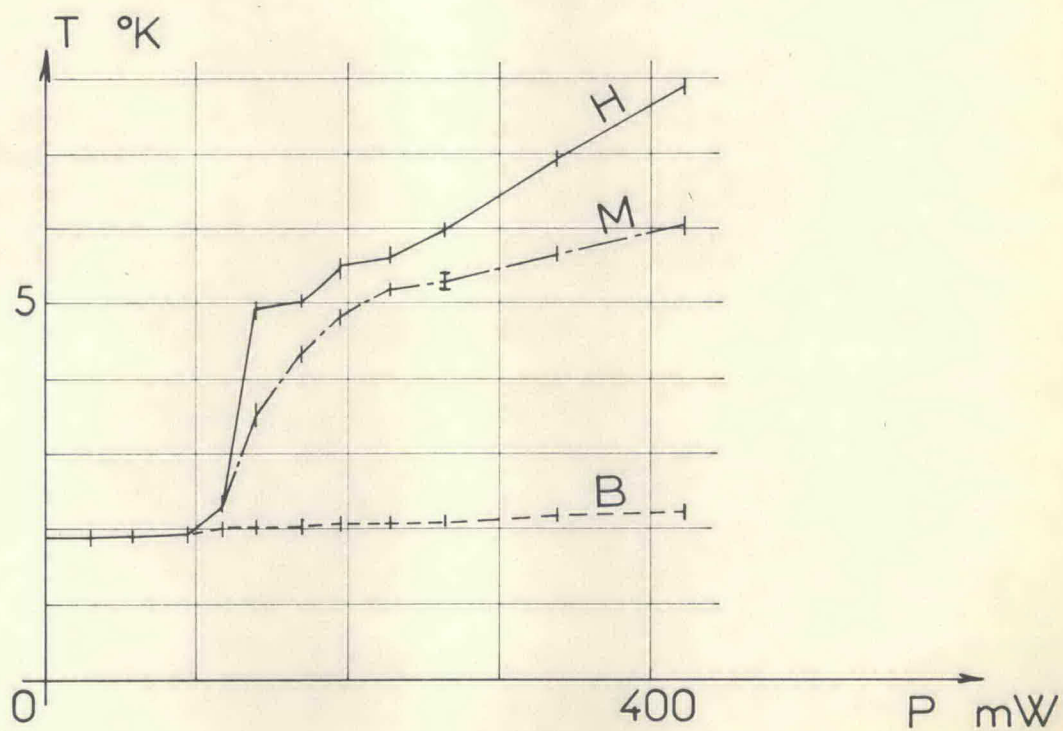
FIG.8 : Superfluid helium T = 1.85 K ; p = 3.5 atm
