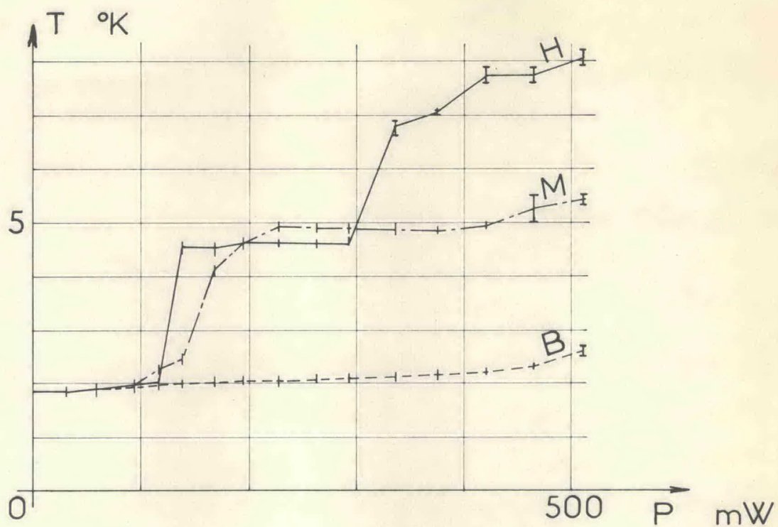
FIG.7 : Superfluid helium T = 1.85 K ; p = 2 atm
